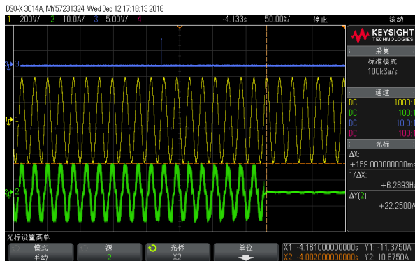
Feed-in current at 25%P
