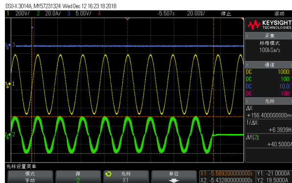
Feed-in current at 50%P
