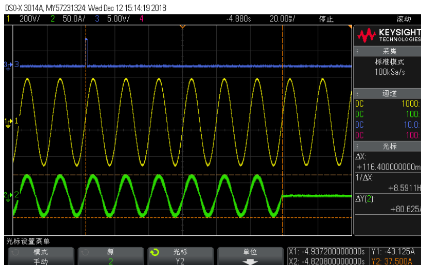
Feed-in current at 100%P
